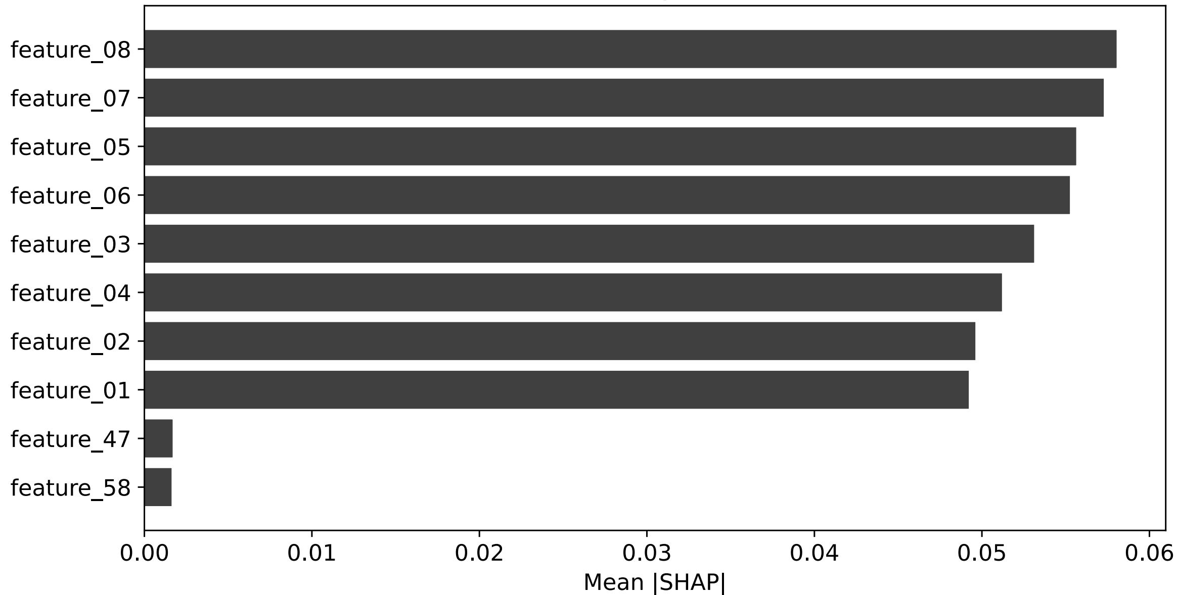
Global feature importance (SHAP)
